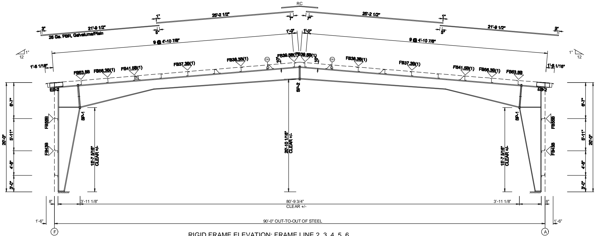
RIGID FRAME ELEVATION: FRAME LINE 2 3 4 5 6
